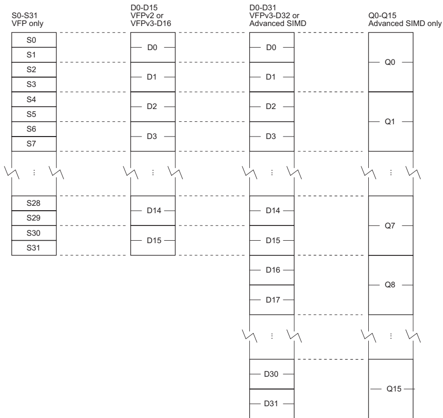
Figure A2-1 Advanced SIMD and VFP register set
