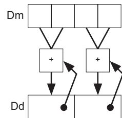
Figure A8-2 Operation of doubleword VPADAL for data type S16
