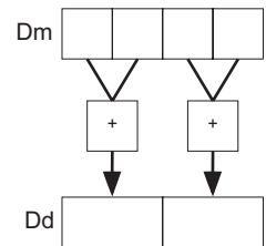
Figure A8-4 Operation of doubleword VPADDL for data type S16
