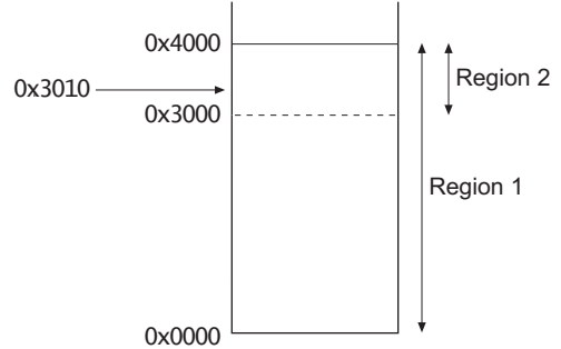
Figure B4-1 Overlapping memory regions in the MPU
