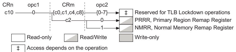
Figure B3-22 CP15 c10 registers
