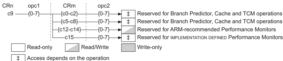
Figure B4-11 Permitted CP15 c9 register encodings
