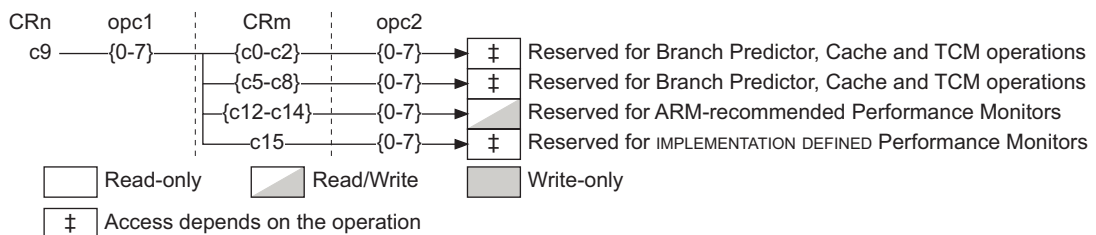
Figure B3-21 Permitted CP15 c9 encodings
